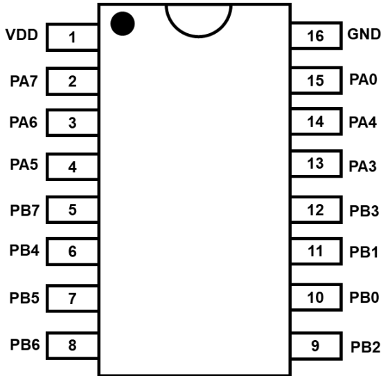
PMS120B-S16A: SOP16 (150mil)
