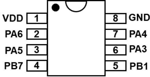
PMS120B-S08A: SOP8 (150mil)
