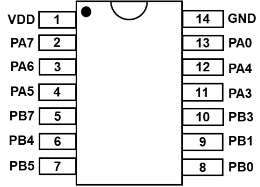
PMS120B-S14A: SOP14 (150mil)
