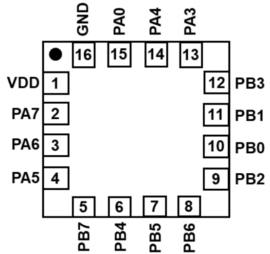
PMS120B-1J16A: QFN3*3-16pin (0.5pitch)
